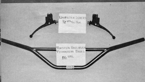
Torsten Hallman titanium handlebars and Unifilter's indestructible polycarbonate levers save about 1 1/2 lb. at an important location on the scooter.
