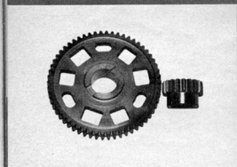
Advance Cycle Engineering's straight-cut gears help the engine last longer and shift better. These are very similar to the YZ gears.
