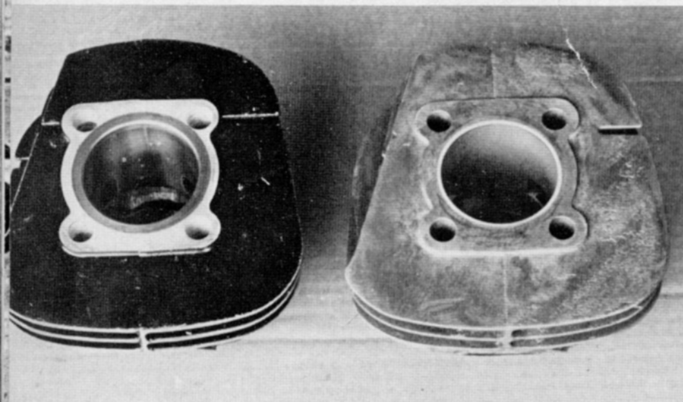
The 1969 GYT Kit aluminum cylinder(right) weighs two pounds less than the standard Yamaha cylinder (left). The GYT Kit cylinder has a chromed barrel, instead of cast iron liner.
