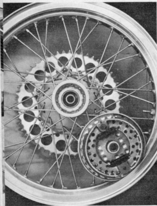
The brake shoes and backing plate of the Rickman rear brake have been drilled to reduce weight, and the aluminum sprocket has been lightened by using a hole saw.
