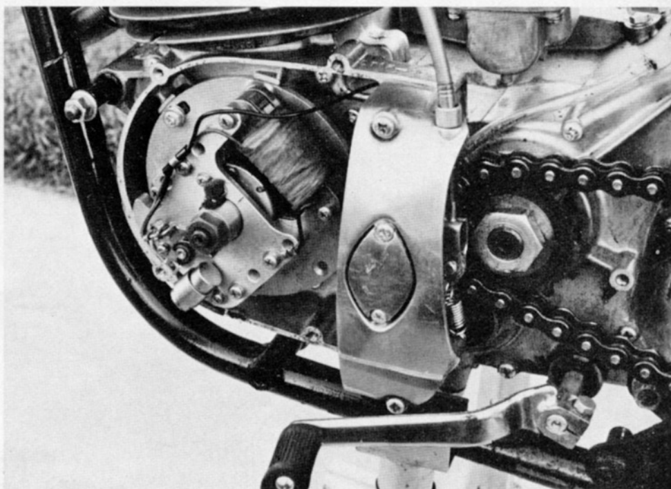
Special machining allowed the installation of this light weight Kawasaki rotor magneto and stator plate. Reduced weight of the crankshaft allows quicker revving of the engine.
