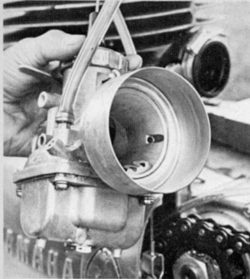
The adaptor fitting by K&N Engineering is essential to allow the 34mm Mikuni road racing carburetor to breathe adequately throughout the entire RPM range.
