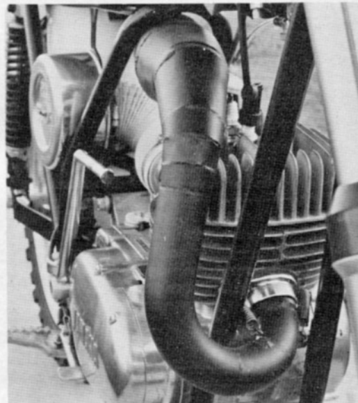
The custom Bassani exhaust pipe fits neatly between the engine and frame and exits at the left rear side. High performance and light weight combine with being out of the way.
